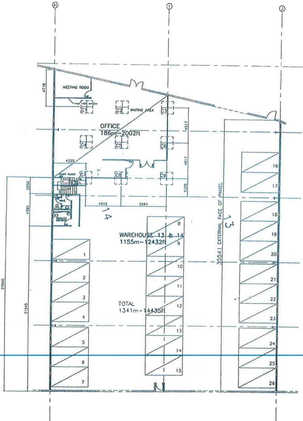
GROUND FLOOR PLAN 1:200
